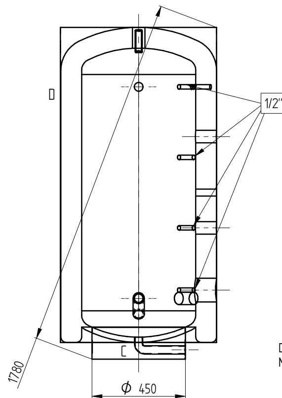
Detail C Drain 1"
